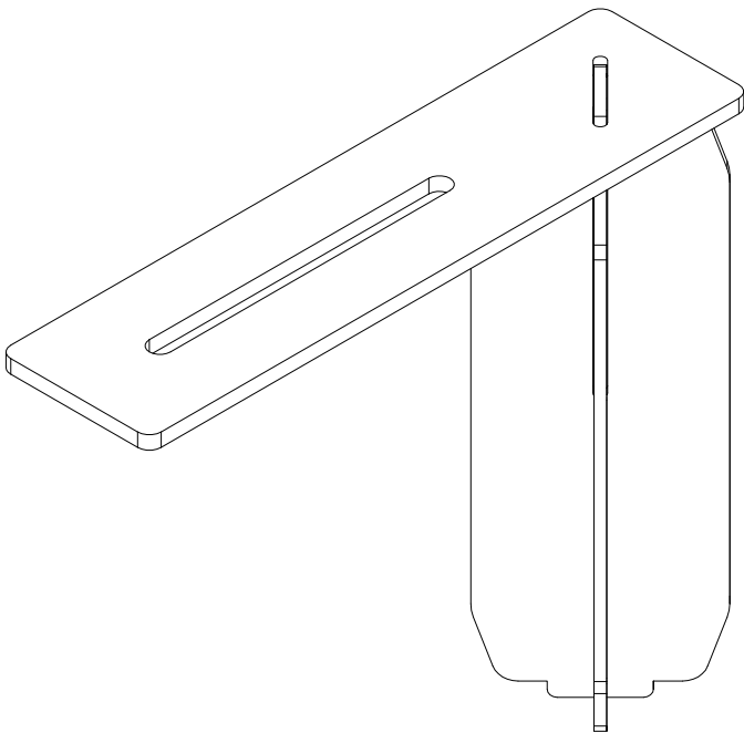
RTCTSRN Cable Tray Support Run
