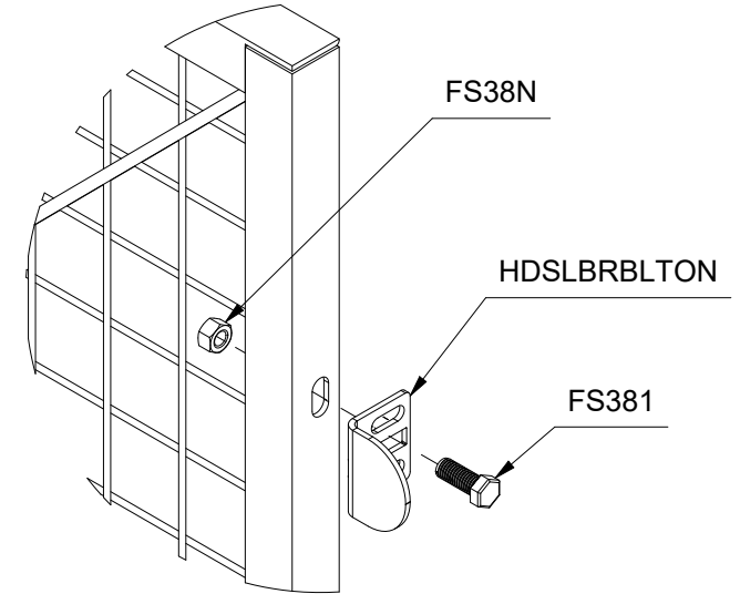
DETAIL SLAM BAR EXPLODED VIEW (TOP & BOTTOM)
