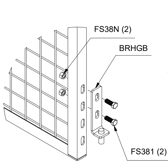
DETAIL HINGE DOOR HINGE BRACKET EXPLODED VIEW
