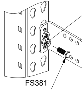
THREAD RETAINING BOLT THROUGH LOWER NUT TO PREVENT BRACKET DISENGAGEMENT
