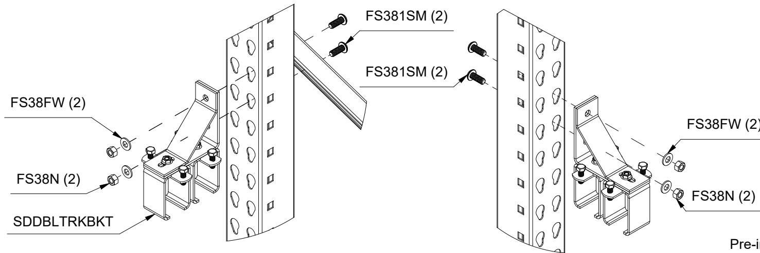
DETAIL SLIDE DOOR LEFT DOUBLE TRACK BRACKET EXPLODED VIEW
