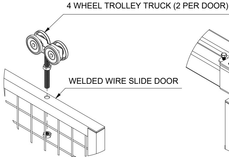
DETAIL TROLLEY TRUCK EXPLODED VIEW
