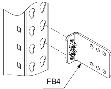
POSITION BRACKET ON RACK UPRIGHT
