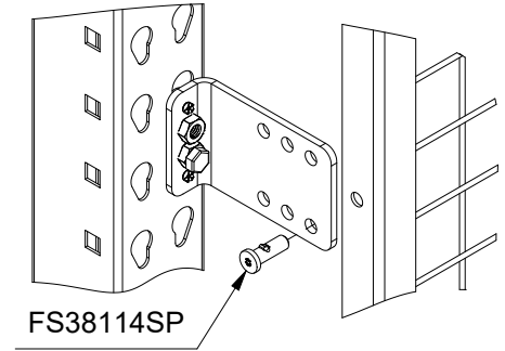
ALIGN PANEL WITH BRACKET AND INSERT PIN UNTIL YOU HEAR A CLICK
