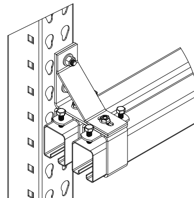
DETAIL SLIDE DOOR LEFT BRACKET W/ SLIDE DOOR TRACKS INSTALLED
