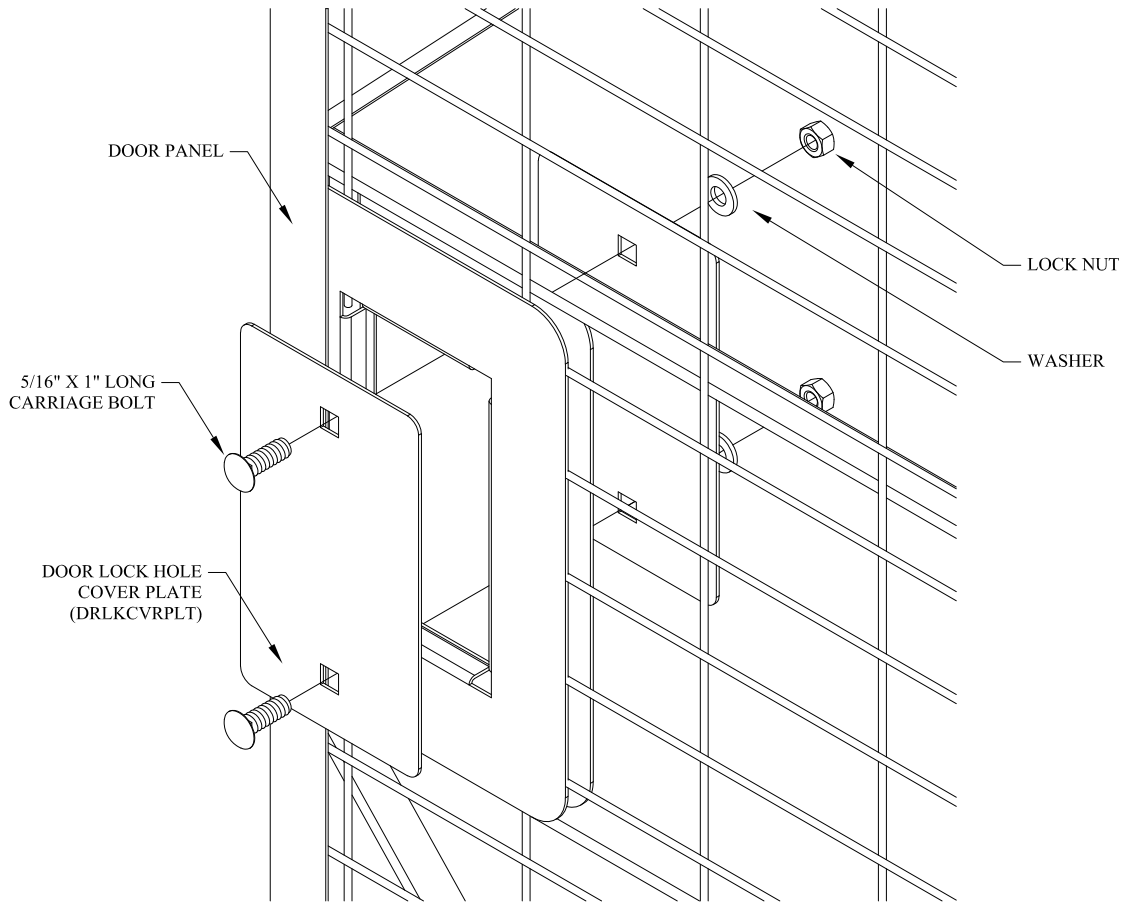
DETAIL COVER PLATE
